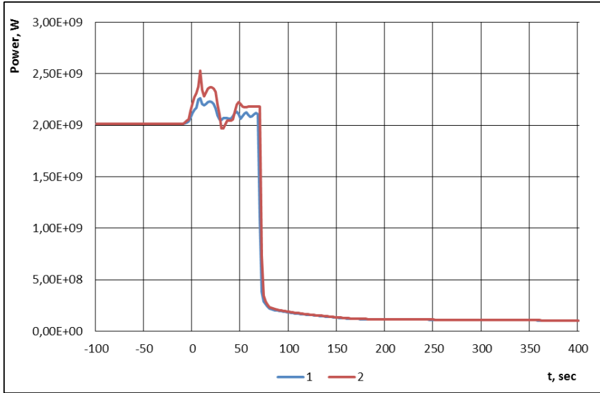
Figure 3 - Reactor power: 1-beginning and 2-end of the campaign.
