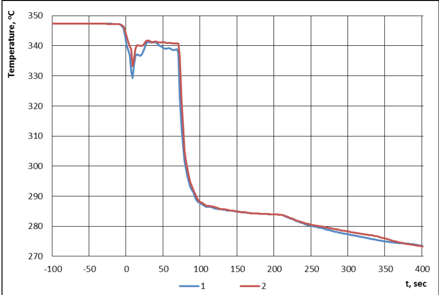
Figure 6 - Maximum shell temperatures: 1-beginning and 2-end of the campaign.
