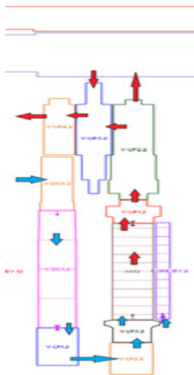
Figure 2 – The flow diagram of the coolant through the reactor.
