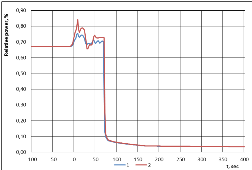
Figure 4 - Relative power: 1-beginning and 2-end of the campaign.
