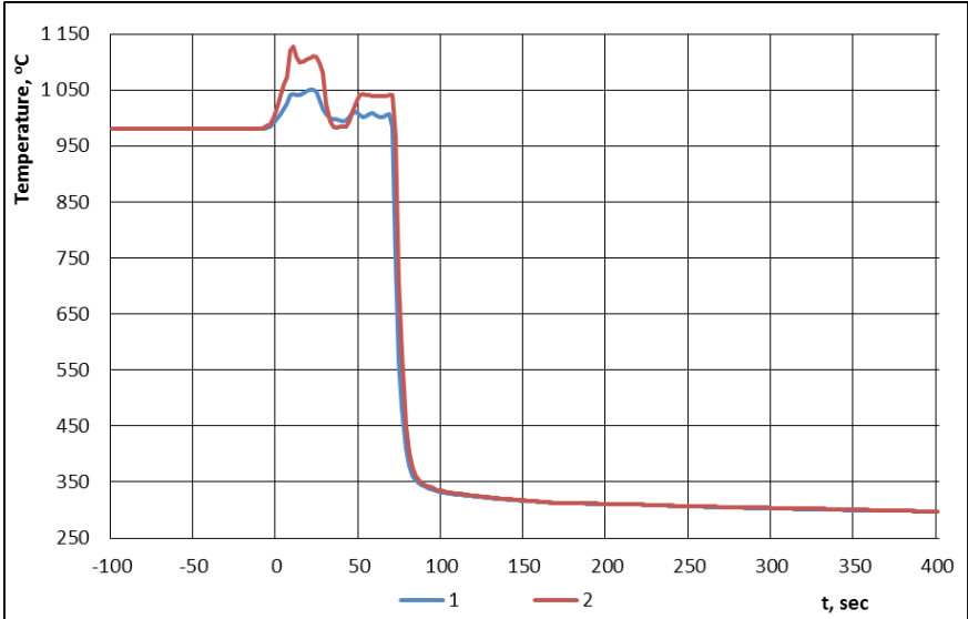
Figure 5 - Maximum fuel temperatures: 1-beginning and 2-end of the campaign.
