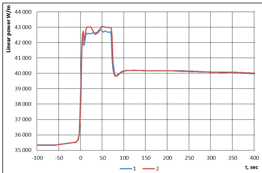
Figure 7 - Heat flow from the surface of a fuel rod: 1-beginning and 2-end of the campaign.
