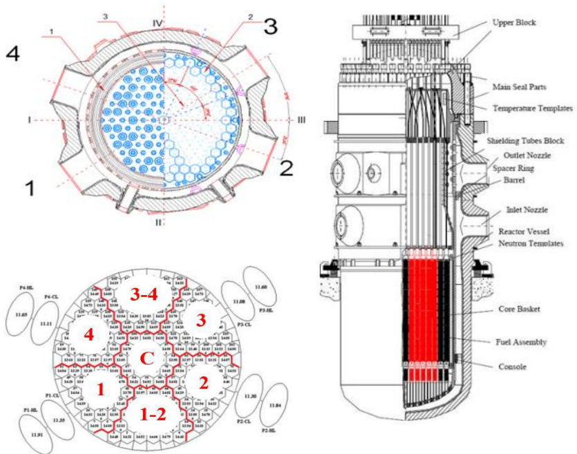
Figure 1. Top left is a diagram of the connection of circulation loops with a reactor; bottom is a diagram of splitting of the core into seven groups of parallel hydraulic channels (six peripheral and one central) and the right diagram of the coolant flow in reactor 3 of the Kalinin NPP unit.
